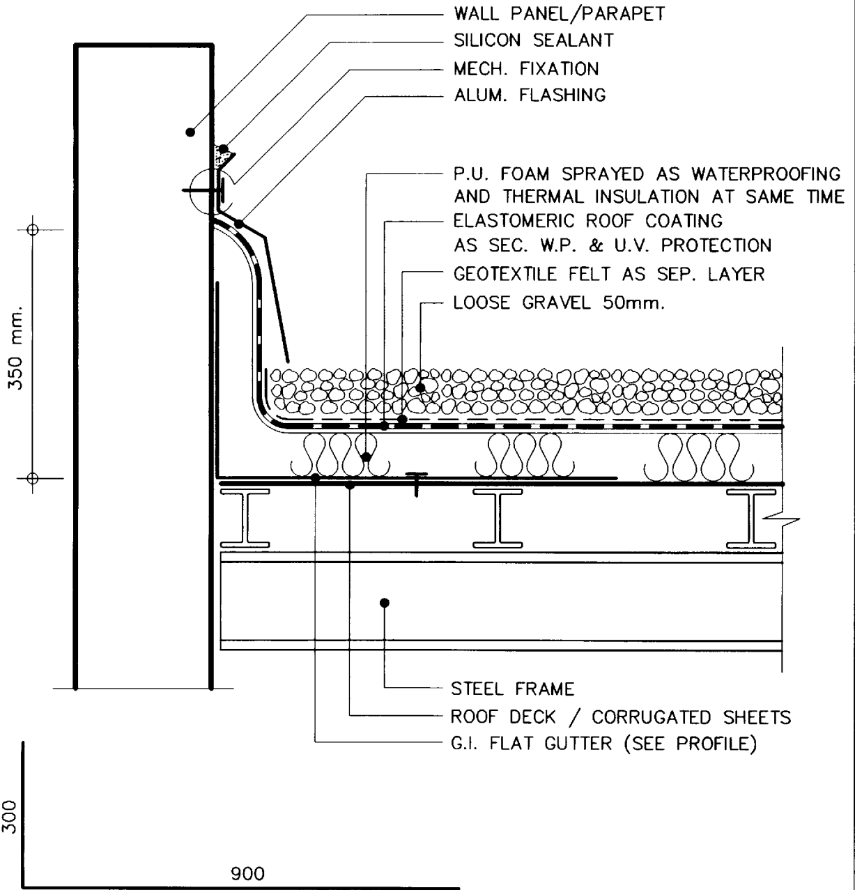
FLAT GUTTER PROFILE
